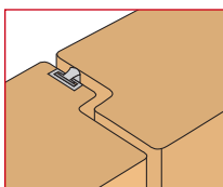
Double action doors (rebated meeting stiles)
