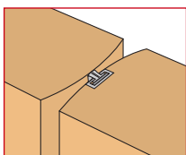
Double action doors (unrebated meeting stiles)
