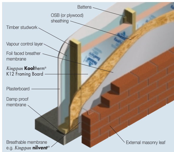
Figure 3 External Masonry – Timber Frame Wall with Insulation Between Studs (Utilising Foil Faced Breathable Membrane)
