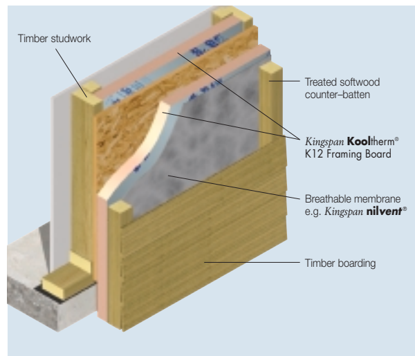
Figure 6 Timber Clad / Tile Hung Timber Frame Wall – Insulation Between Studs and Insulating Sheathing
