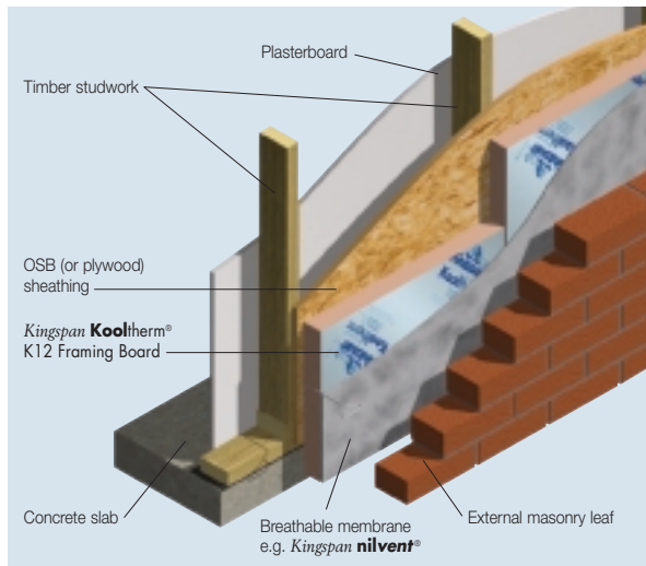
Figure 1 External Masonry – Timber Frame Wall with Insulating Sheathing
