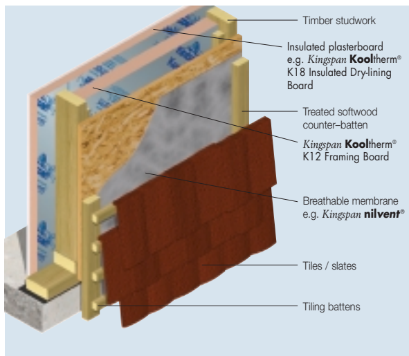
Figure 5 Timber Clad / Tile Hung Timber Frame Wall – Insulation Between Studs and Insulated Dry-lining
