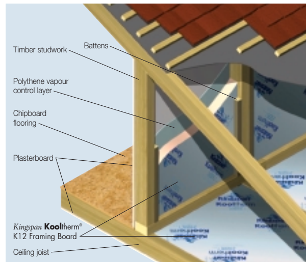
Figure 4 Dwarf Wall – Insulation Between Studs
