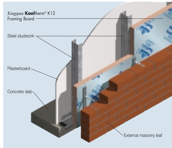
Figure 2 External Masonry – Steel Frame Wall with Insulating Sheathing
